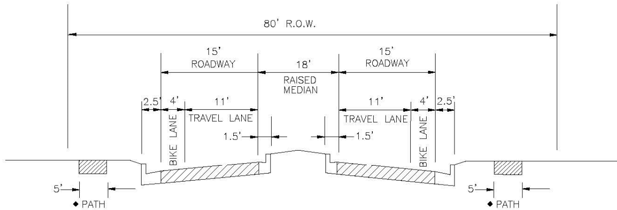
COLLECTOR WITH RAISED MEDIAN
