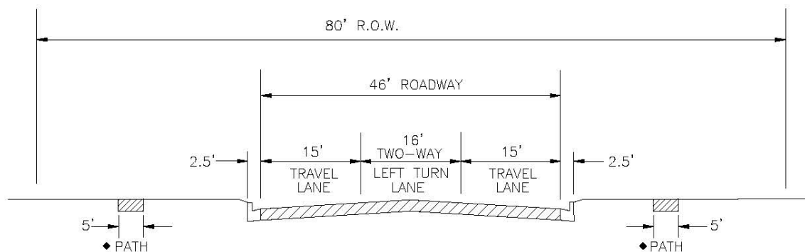
COLLECTOR WITH FLUSH MEDIAN (PRIMARILY INTENDED FOR INDUSTRIAL AREAS)
