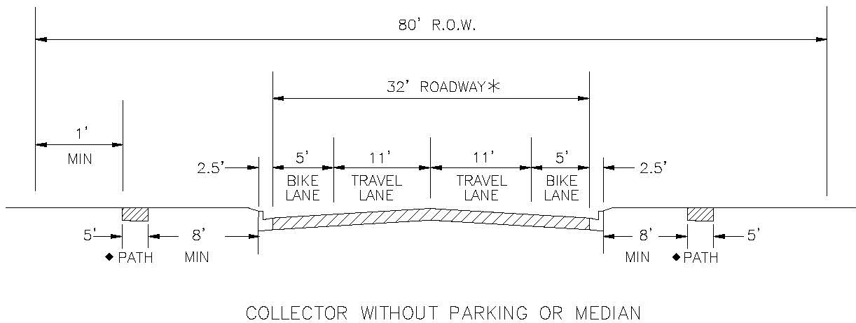
Figure 21. Collector Without Parking or Median
