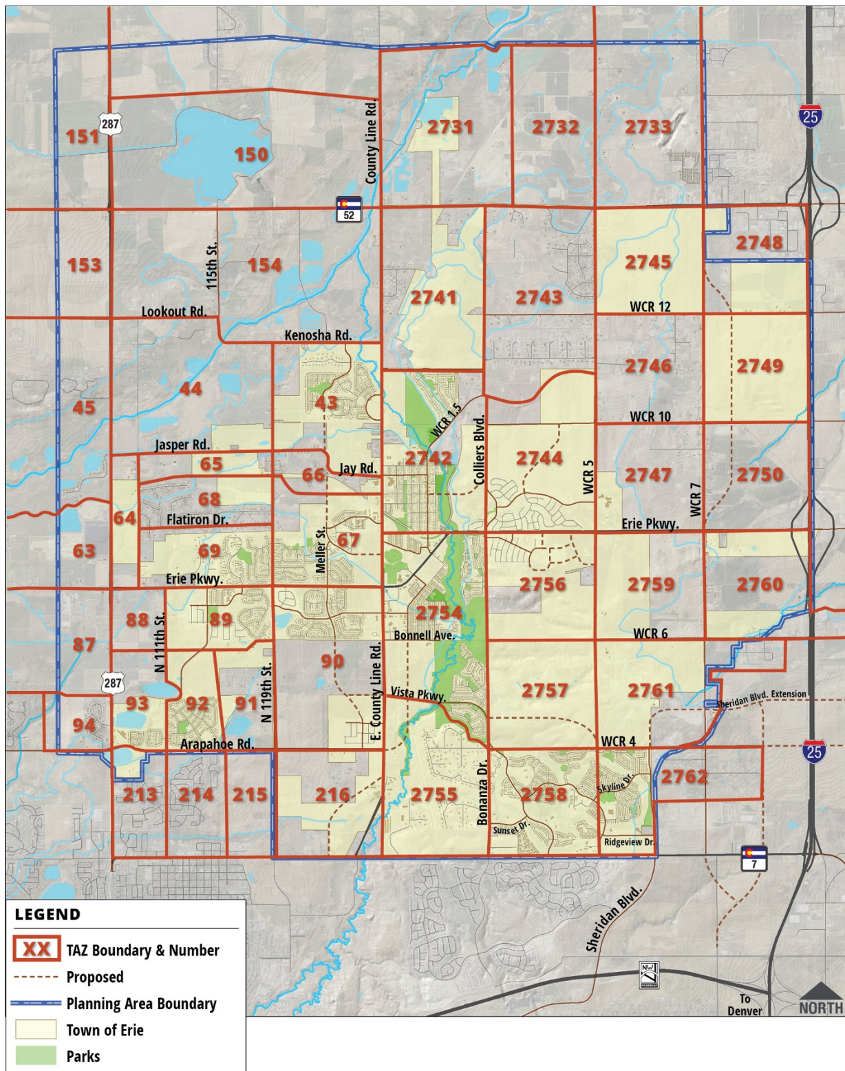
Figure 12. DRCOG Traffic Analysis Zones (TAZs)
