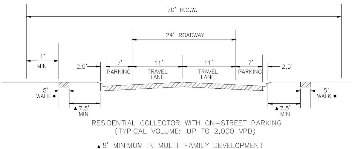
Figure 22. Residential Collector With On-Street Parking
